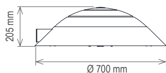
Fixation suspendue
