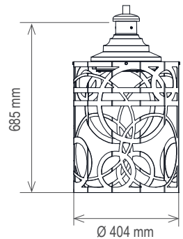
Fixation suspendue
