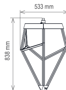
Fixation suspendue
