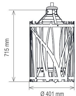
Fixation suspendue
